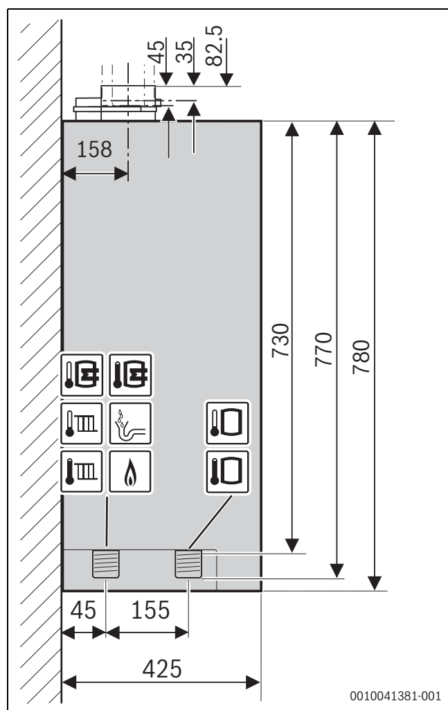
Obr. 3 Pohled z boku GB192i.2 15-25-35 kW(T40S) (mm)
